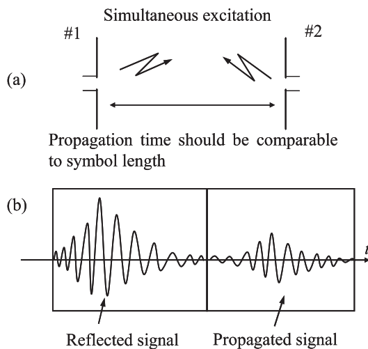
Fig. 2 Sketch of the antennas and signals in the analysis that uses the CI method: (a) conceptual sketch of the antennas, (b) observed time domain signal.
