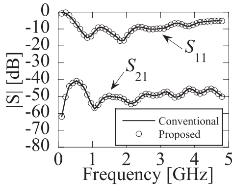
Fig. 9 Comparison of simulated scattering parameters between conventional method and proposed method using CI technique ( D/L = 2.0 ).
