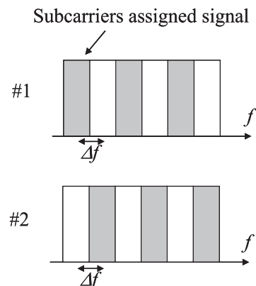
Fig. 1 Signal arrangement.
