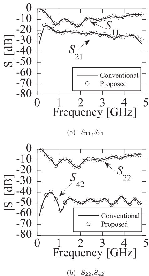
Fig. 12 Comparison of simulated scattering parameters yielded by conventional method and proposed method using combined OFDM and CI technique ( D/L = 2.0 ).
