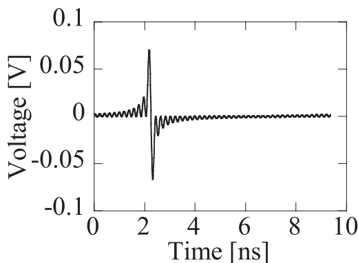
Fig. 7 CI pulse waveform.
