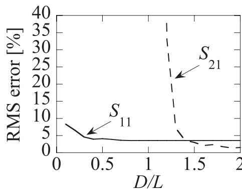
Fig. 8 RMS error between conventional method and proposed method using CI technique.
