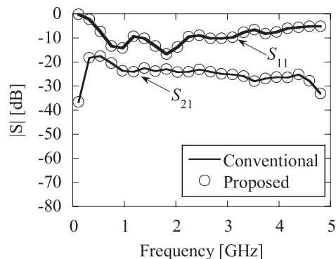
Fig. 6 Comparison of the simulated scattering parameters: conventional method and proposed method using OFDM technique ( D/L = 0.05 ).
