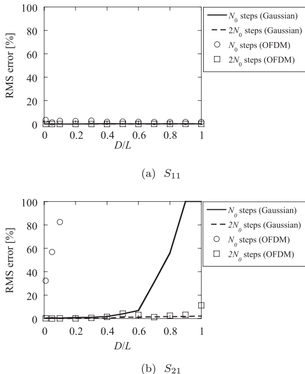
Fig. 5 RMS error of scattering parameter versus antenna distance, D , in OFDM technique.
