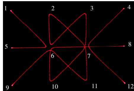
(b) Without drawing order optimization: the drawing order is (8,7,6,10,7,3,6,2,7,11,6,9,5,6,1,4,7,12,8)
