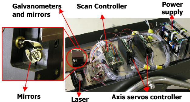
Figure 6: Experimental laser projector
