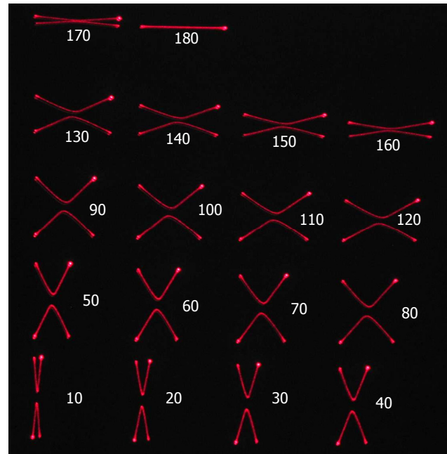
Figure 9: Undesired inertia effect in different angles
