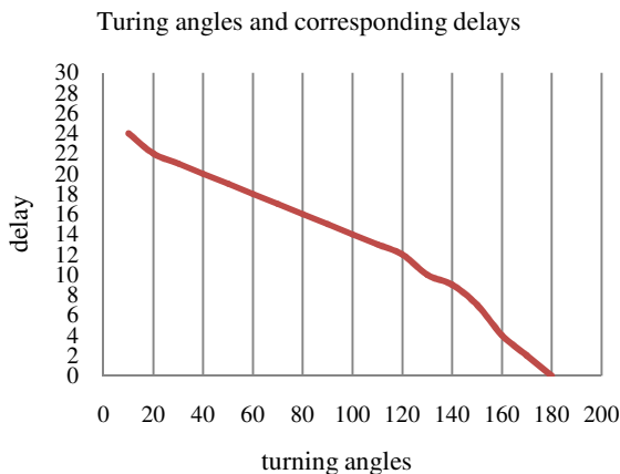
Figure 11: Relation between demanded delays and angles
