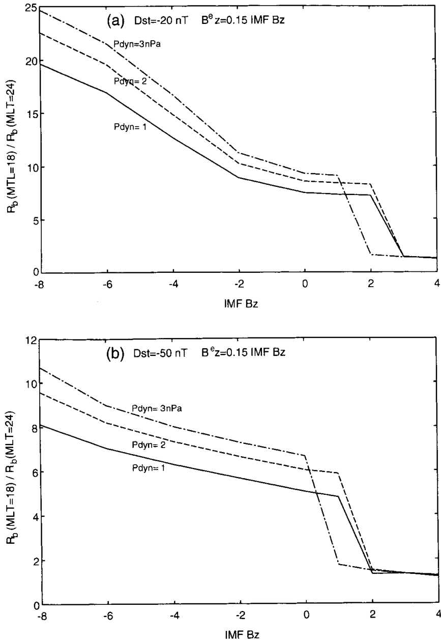
Fig. 10. Ratio between the two values of R_b at \text{MLT}=18 and 24 hours, on the same \kappa=1 line, plotted against \text{IMF } B_z for P_{\text{dyn}}=1, 2 and 3 nPa in the cases of (a) D_{\text{ST}}=-20 nT and (b) D_{\text{ST}}=-50 nT; B_z^e=0.15 \times \text{IMF } B_z .
