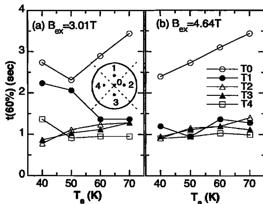
Fig. 3. The t(60\%) value at the positions (P0~P4) as a function of the initial stage temperature T_s for (a) B_{ex} = 3.01 and (b) 4.64 T.
