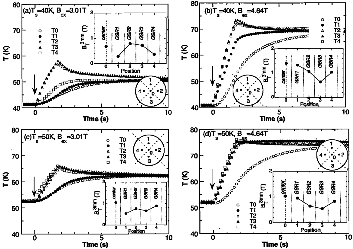
Fig. 2. The time evolution of temperatures T0(t) \sim T4(t) for P0~P4 at T_s = 40 K after applying the pulse field of (a) 3.01 T and (b) 4.64 T, respectively. (c) and (d) show T0(t) \sim T4(t) at T_s = 50 K after applying the same pulse fields as (a) and (b), respectively. The insets of figures present the B_T^{3\text{mm}} values at each position.
