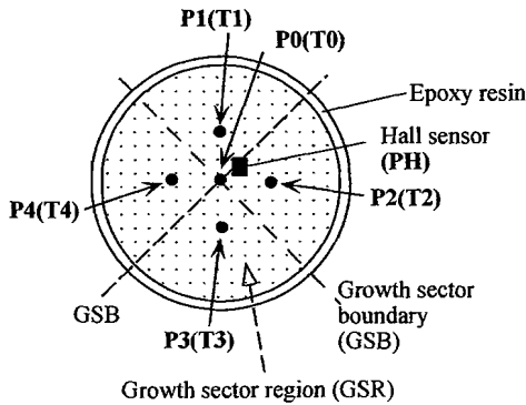
Fig. 1. The positions for the temperature and trapped field measurements on the surface of the SmBaCuO bulk. P0–P4 for the temperature measurement of T_0 - T_4 are indicated. The trapped fields B_T^{3\text{mm}0} - B_T^{3\text{mm}4} are also measured at 3 mm just above P0–P4 by a scanning Hall sensor. The trapped field B_T on the bulk surface is measured using a fixed Hall sensor at PH.
