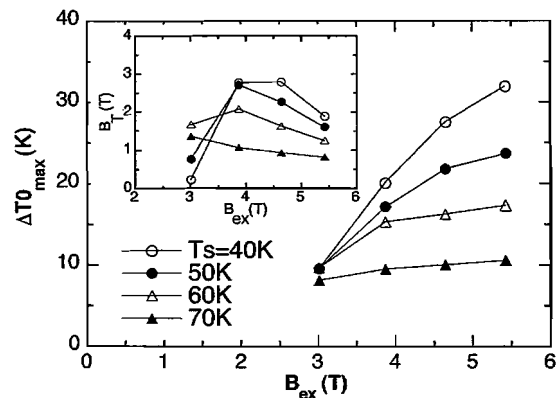
Fig. 4. The maximum temperature rise \Delta T0_{max} at P0 for each T_s as a function of B_{ex} . The inset presents the B_{ex} dependence of B_T monitored by the Hall sensor fixed at PH shown in Fig. 1.
